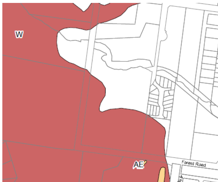
Figure 18 - Extract from PLEP 2014 Geotechnical Hazard Map
