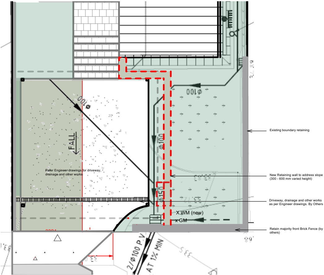
Hardscape Plan (Red showing Landscape works to complete)
