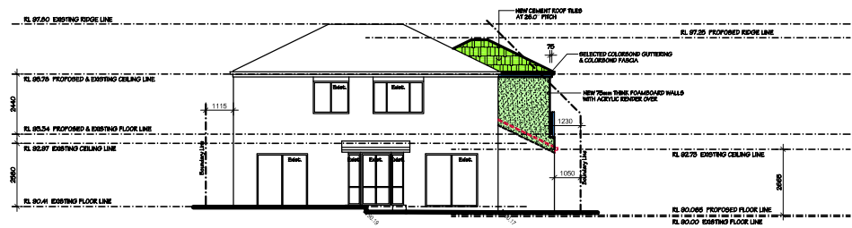
NORTH-EASTERN ELEVATION - REAR NOT TO SCALE
