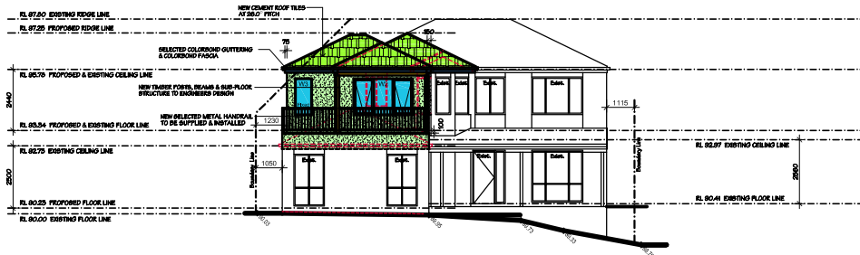
SOUTH-WESTERN ELEVATION - FRONT NOT TO SCALE
