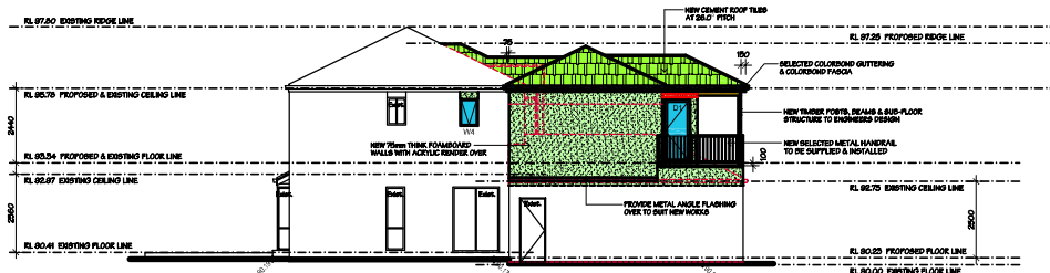
NORTH-WESTERN ELEVATION - SIDE NOT TO SCALE
