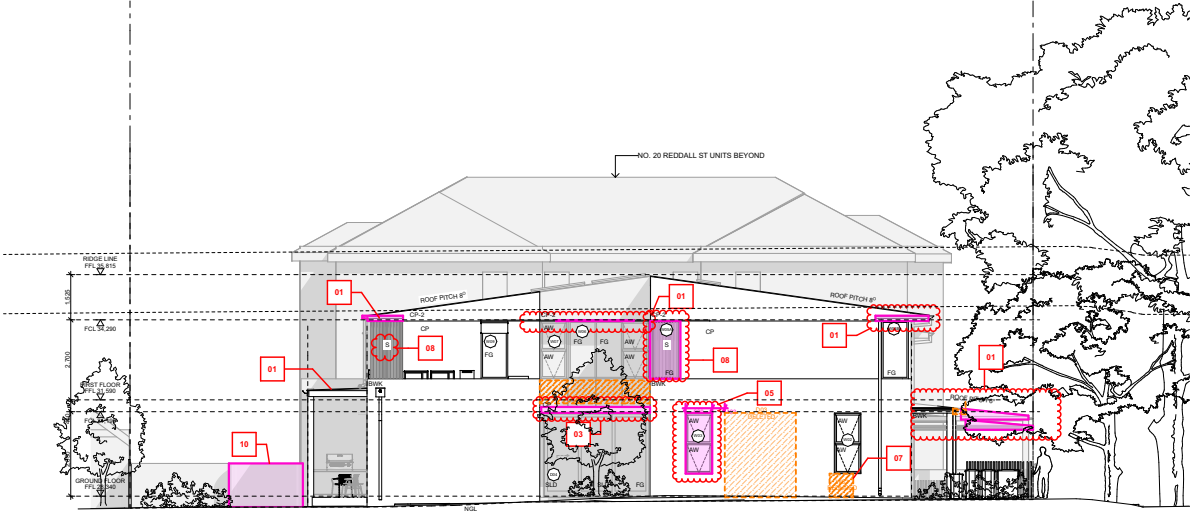
WEST ELEVATION | 1:250
