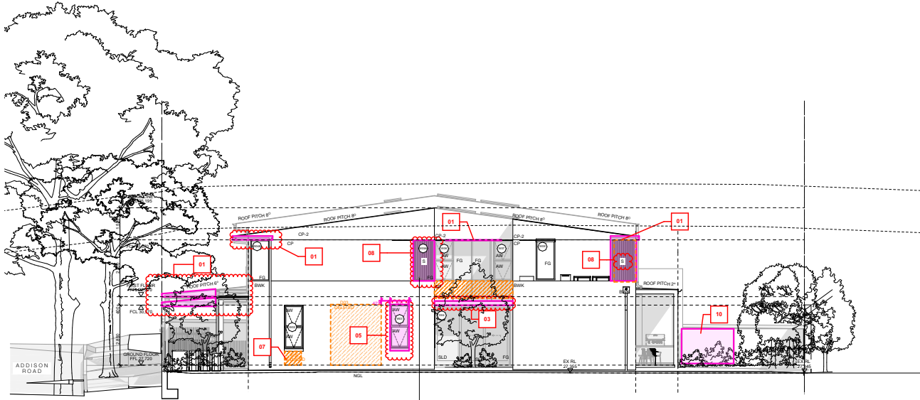
EAST ELEVATION | 1:250
