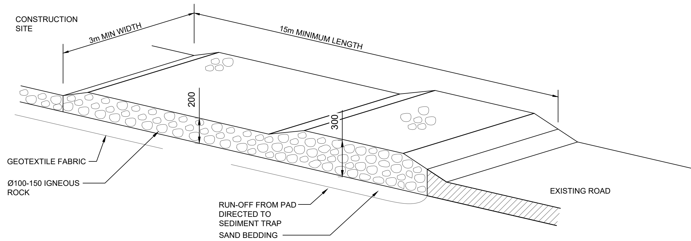
RUBBLE ALTERNATIVE
