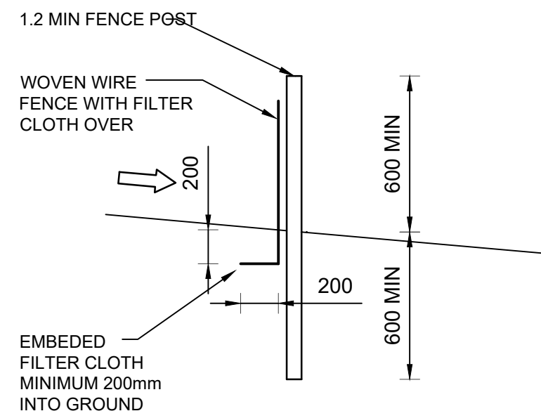
TYPICAL SECTION
