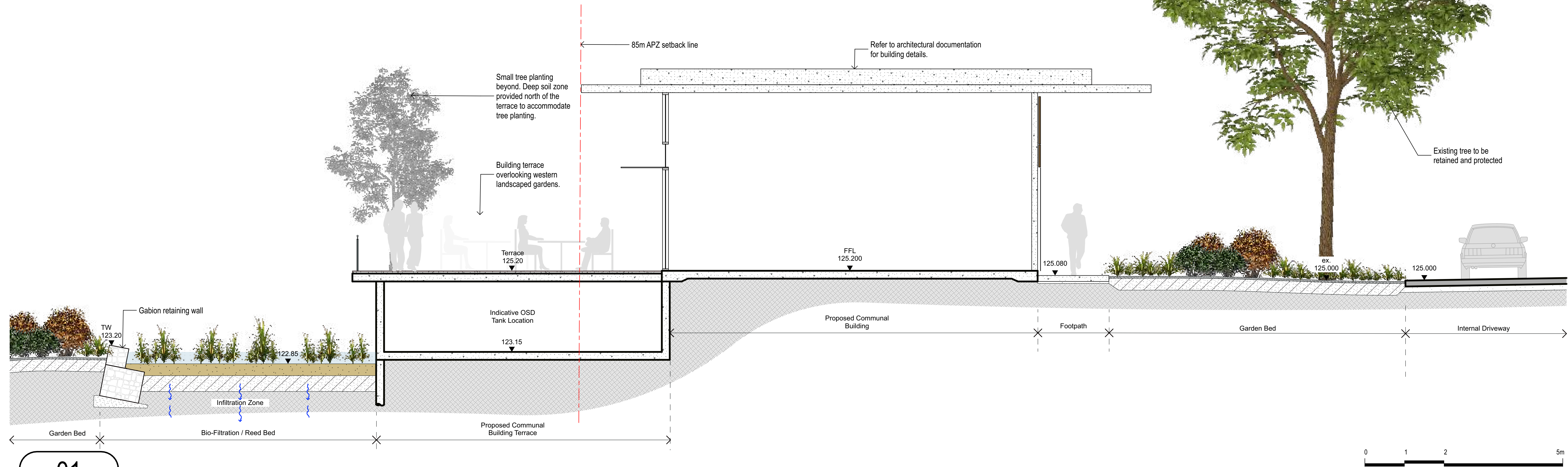
Section BB - Communal Building, Terrace and Tiered Garden Beds
