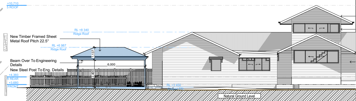
North 1:200
