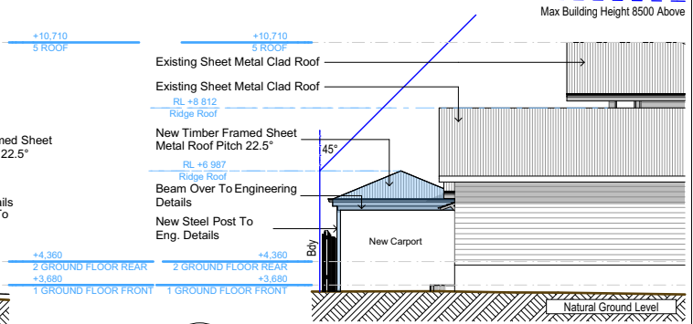
West 1:200
