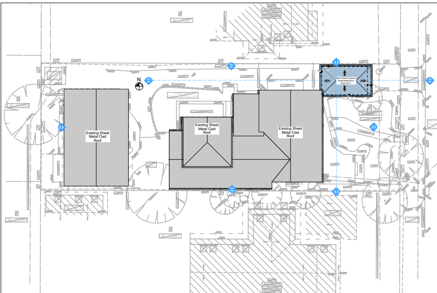
Roof Plan 1:500
