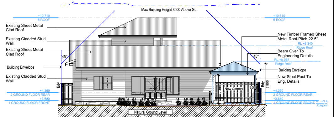
East 1:200
