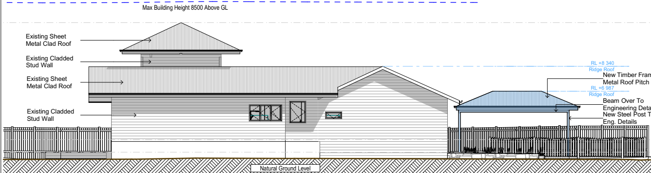
South 1:200
