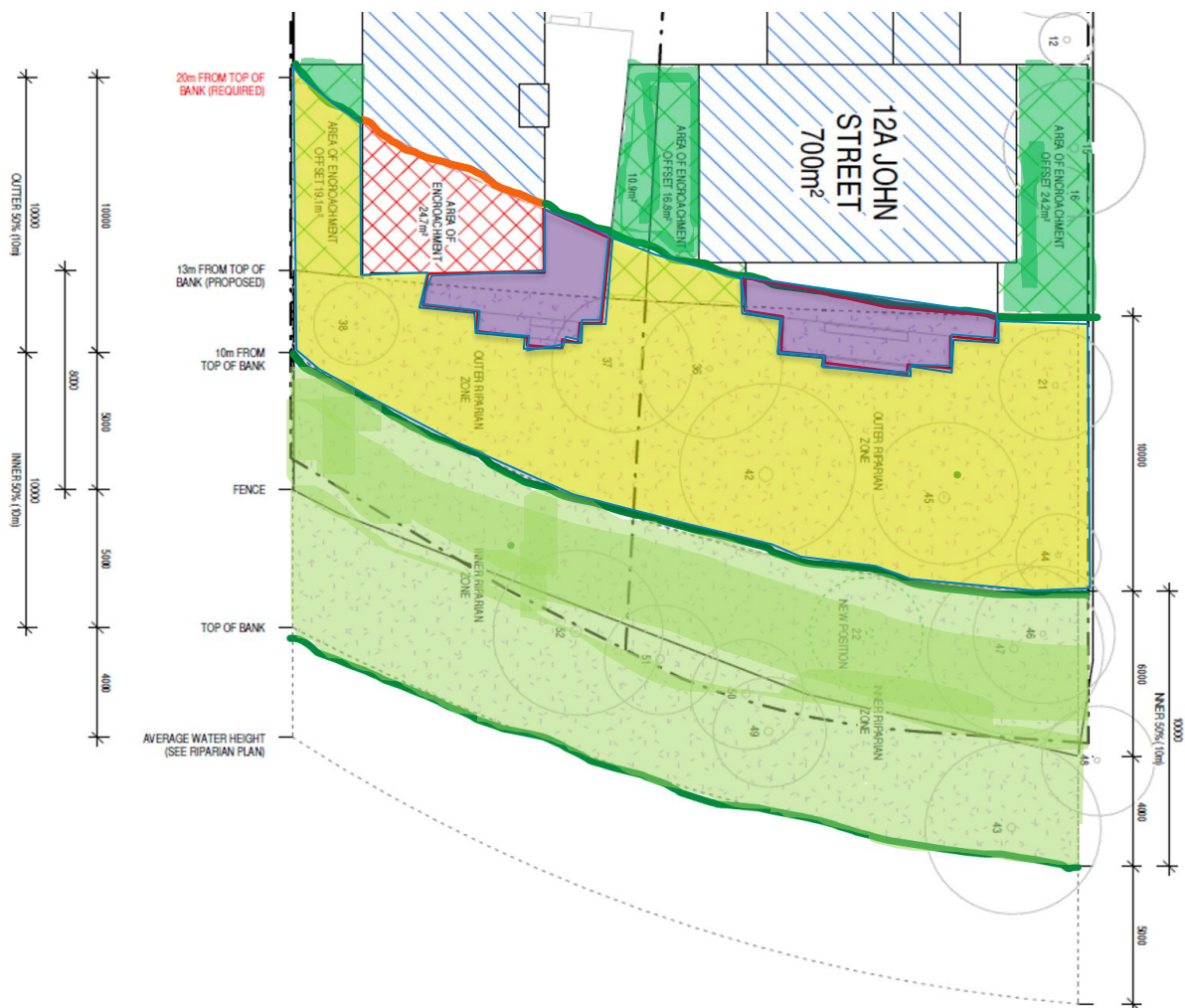
Figure 3.2. Riparian area, top of bank and building footprint overlay.
