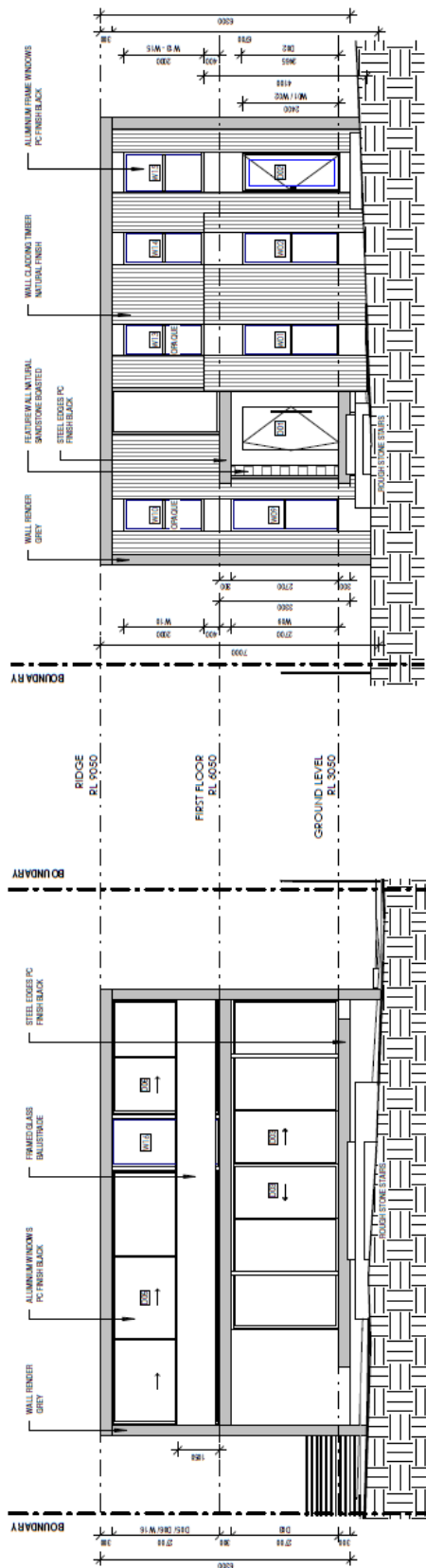
2 WEST ELEVATION
