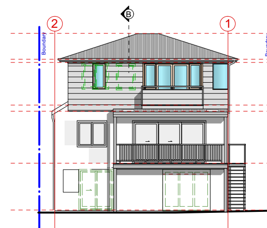
4 East Elevation Scale 1:200
