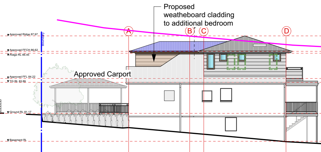
1 South Elevation Scale 1:200
