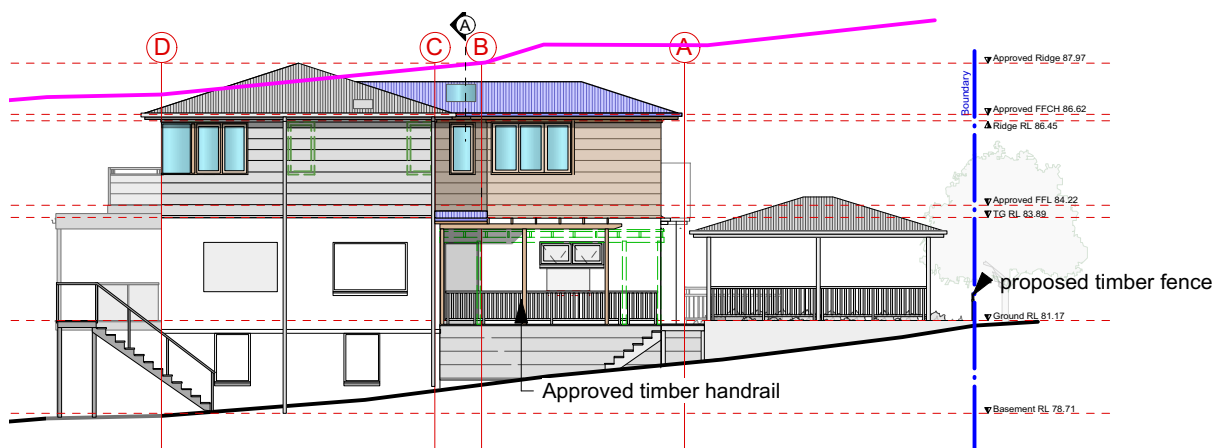
1 South Elevation Scale 1:200
