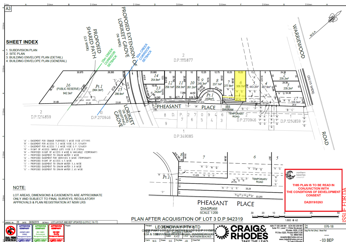
Figure 2 – Approved Subdivision Plan DA2019/0263 with Lot 6 highlighted in yellow Source: Northern Beaches Council
