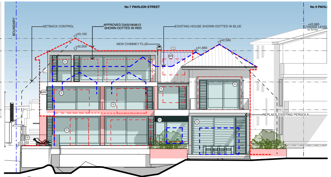
East Elevation 1:200
