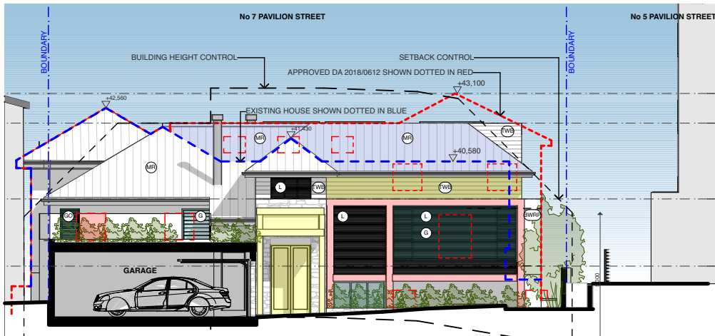
West Elevation 1:200
