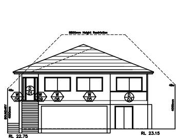
EAST ELEVATION
