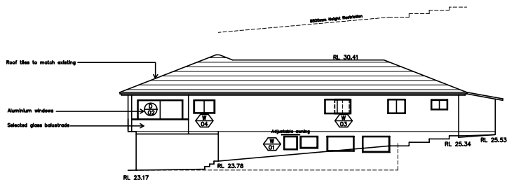
NORTH ELEVATION
