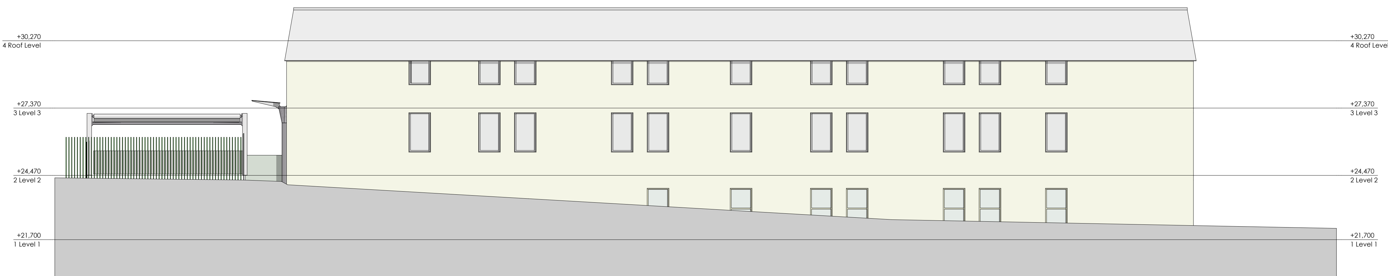
SOUTH ELEVATION
