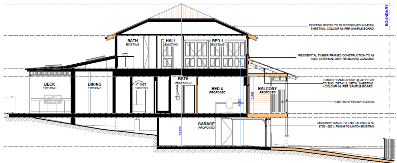
Figure 1. Plan Extract: 1. Long Section illustrating maximum building height.
