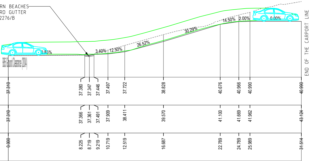
SEC B LOT 2 DRIVEWAY- CENTER LINE ALIGNMENT 1:200
