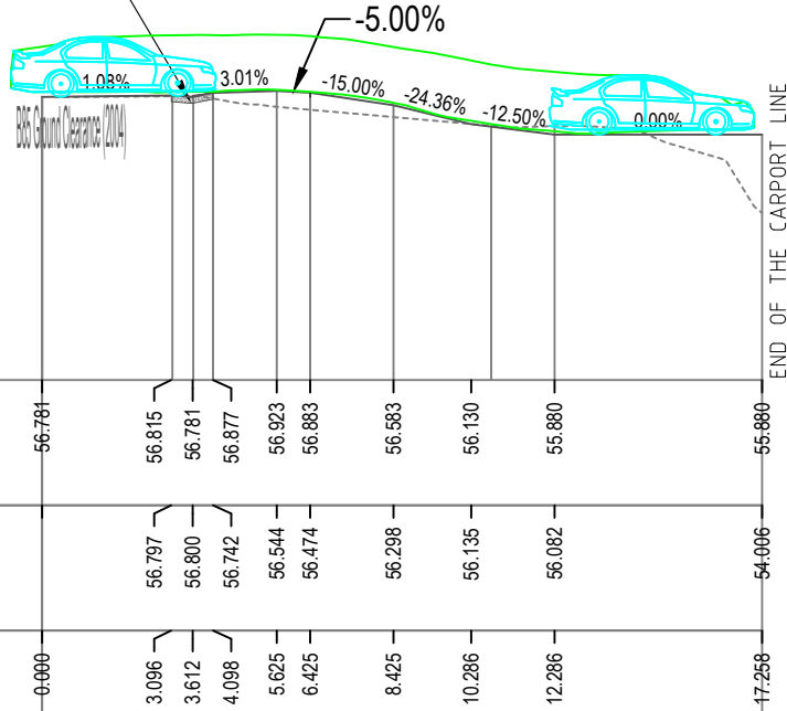
SEC A LOT 1 DRIVEWAY- CENTER LINE ALIGNMENT 1:200
