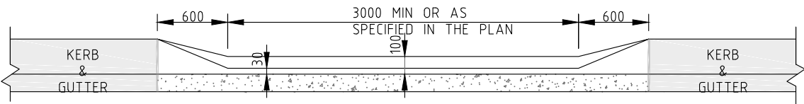
TYPICAL ELEVATION AT KERB FACE
