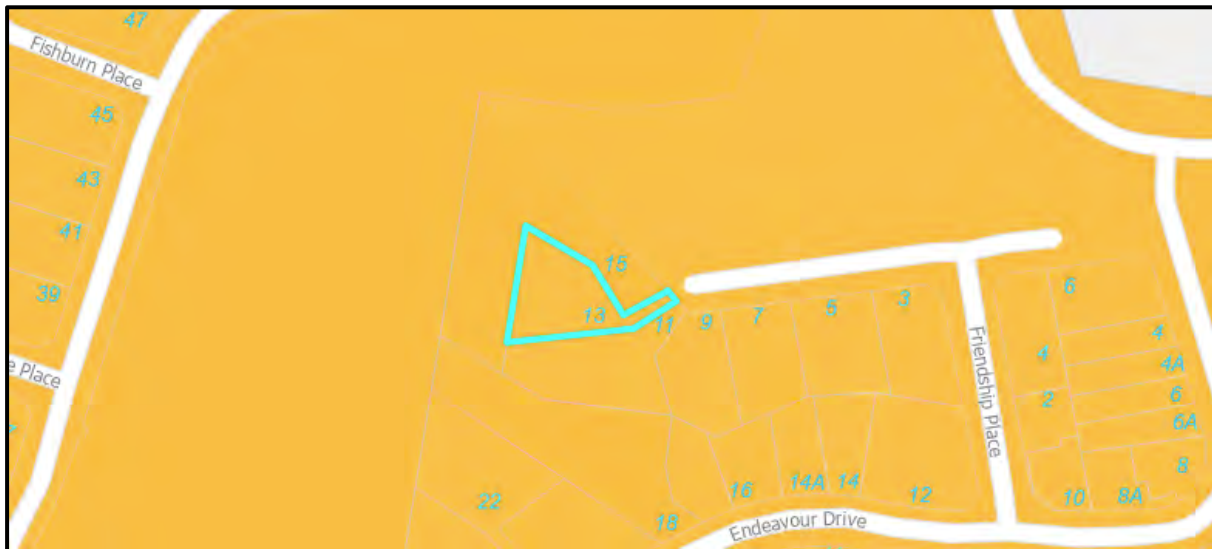
Figure 1. Warringah Landslip Risk Map: 13 Friendship Place, Beacon Hill NSW (© NBC Maps)
