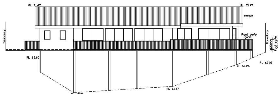
○ WEST ELEVATION Facing McCarr's Creek Road
