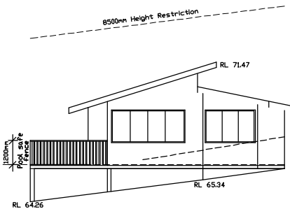
○ SOUTH ELEVATION
