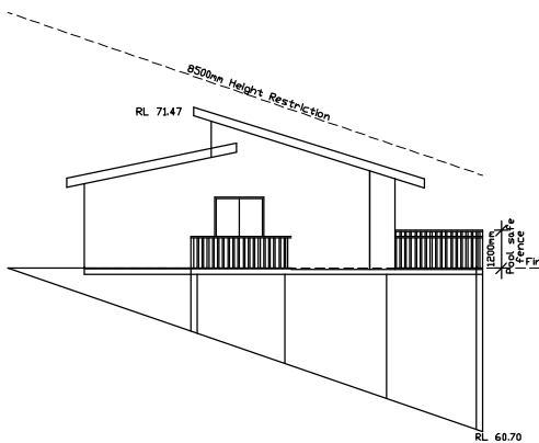
○ NORTH ELEVATION
