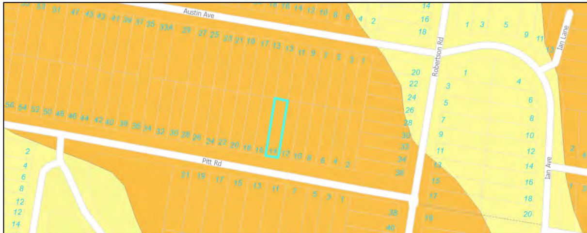
Figure 1. Warringah Landslip Risk Map: 14 Pitt Road, North Curl Curl NSW (© NBC Maps)
