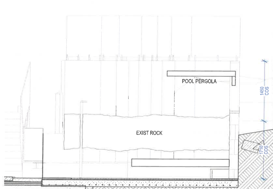
B ELEVATION OF POOL DECK 1:50
