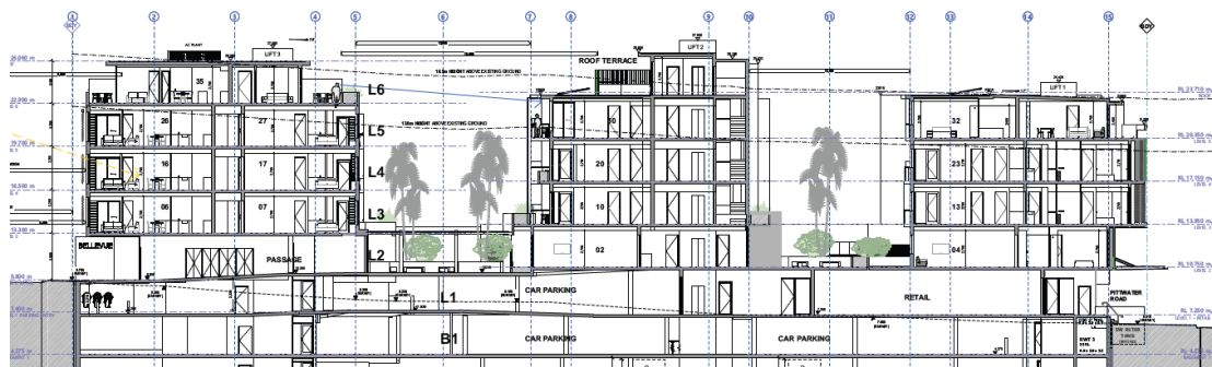
Figure 1 - Section extracts with the 16.9m building height line plotted and non-complying elements depicted above (Source: Gartner Trovato)
