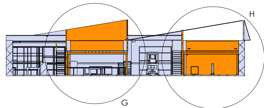
SECTION F-F
