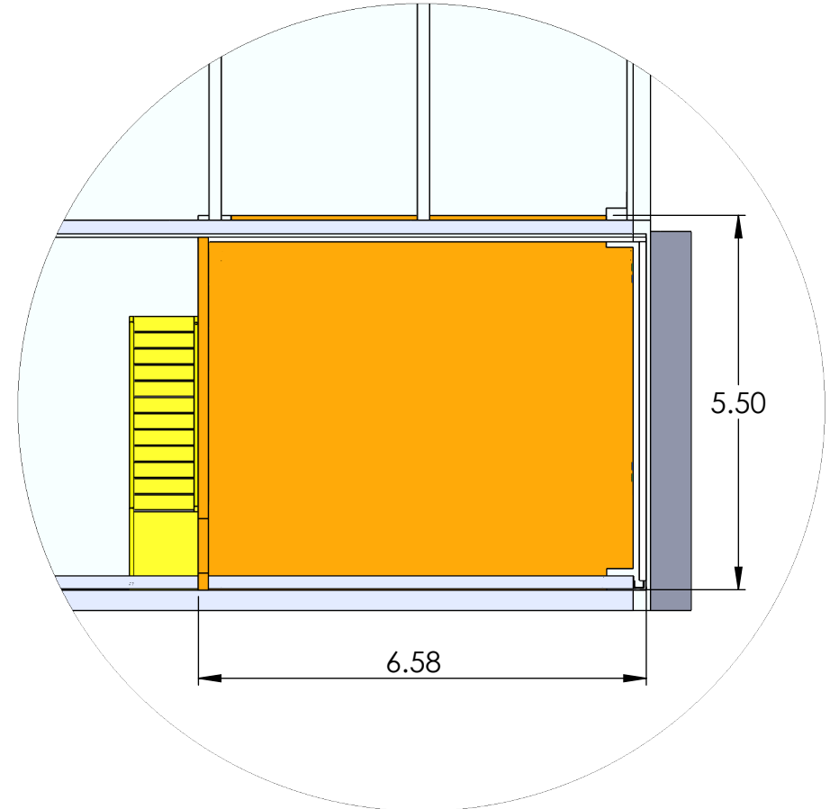
DETAIL E SOUTH MEZZANINE SCALE 1 : 100
