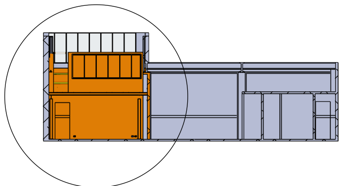
SECTION I-I
