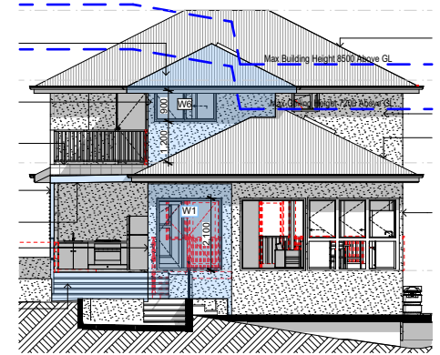
E-03 South 1:200
