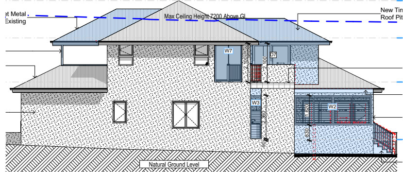
E-04 West 1:200
