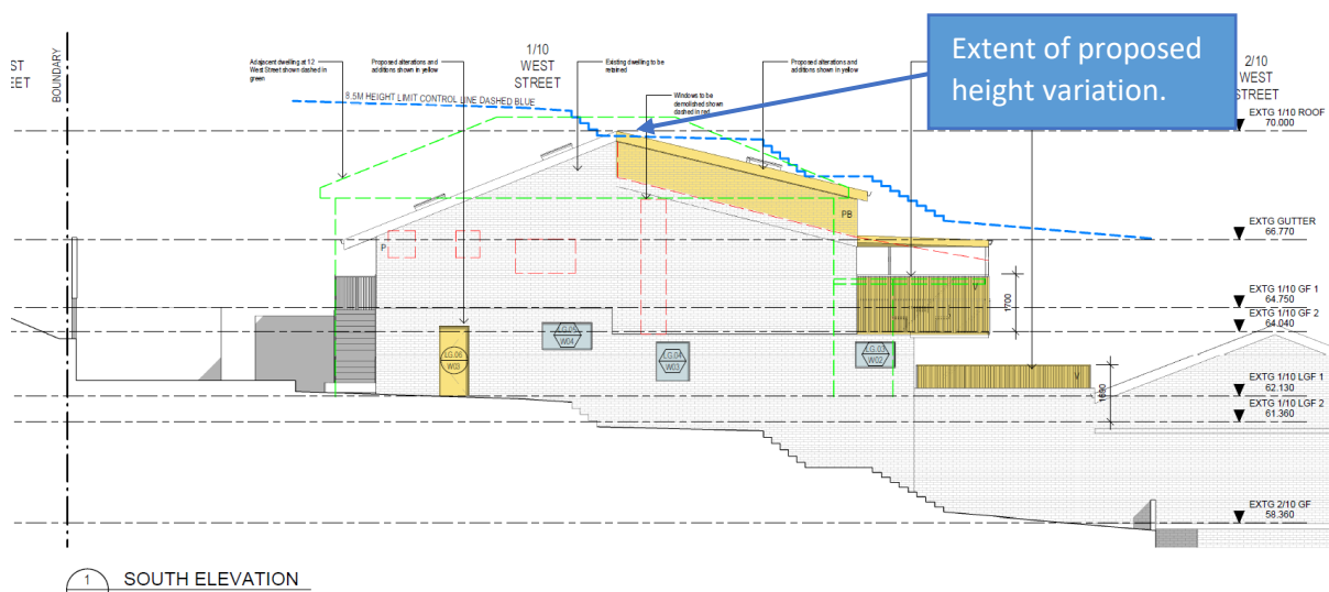
Figure 1: Extract from architectural plans shows the extent of the proposed variation.
