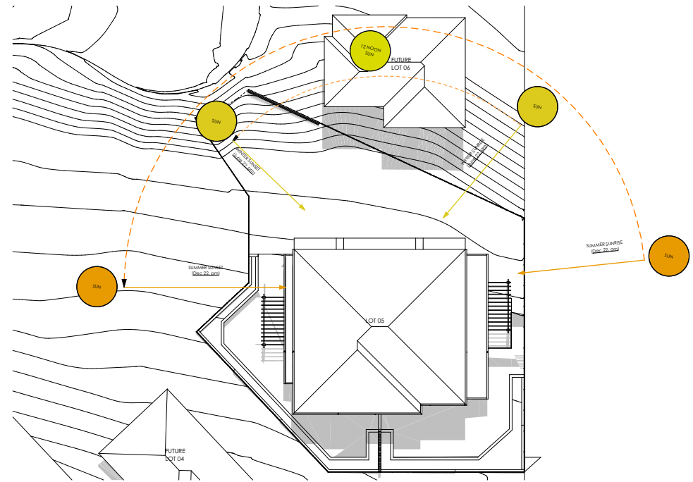
5 SITE ANALYSIS PLAN 1:500
