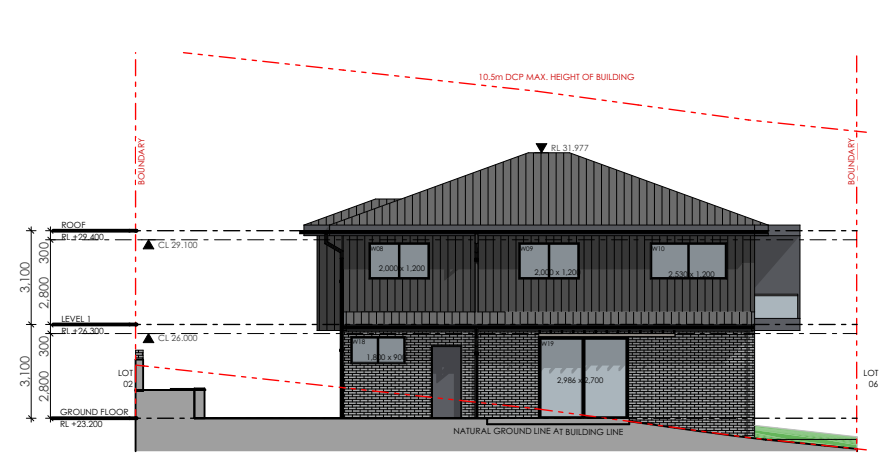
2 EAST ELEVATION 1:250
