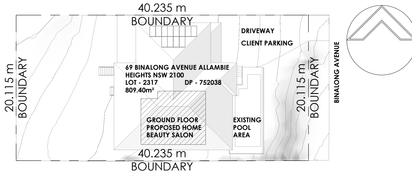
SITE PLAN
