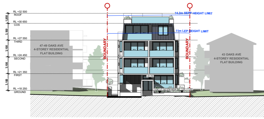
NORTH ELEVATION
