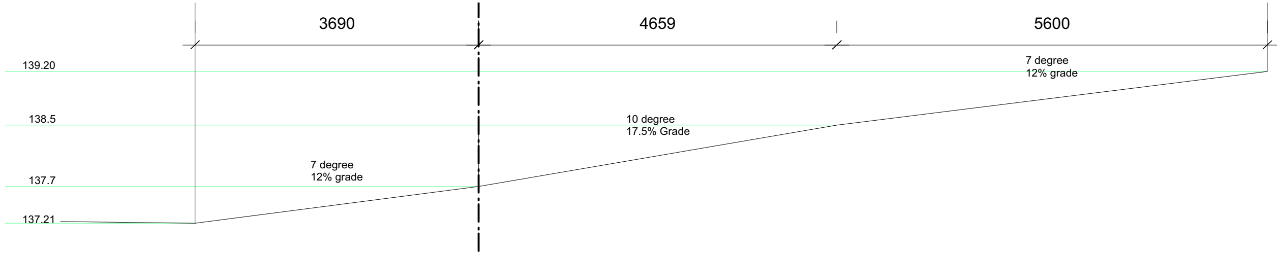
Driveway profile 1:50@A1 1:100@A3.
