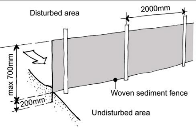
Sedimentation Control Fence Not to scale.
