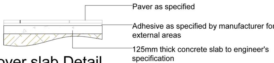
Pave over slab Detail 1:20. Do not scale off plan
