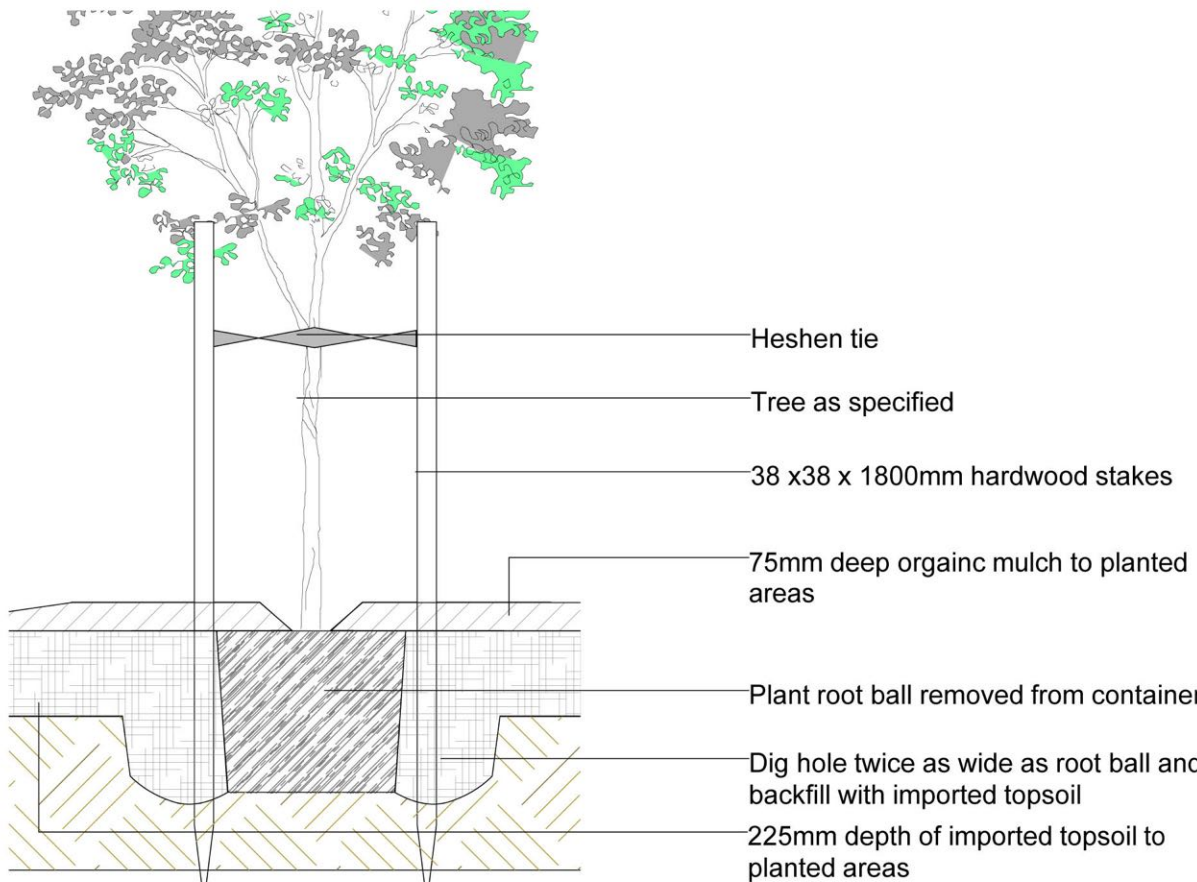
Tree Planting Detail 1:20. Do not scale off plan
