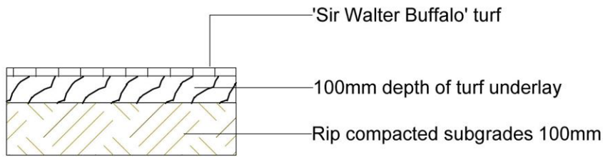
Turf detail 1:20. Do not scale off plan
