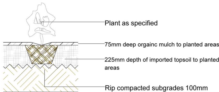
Shrub Planting Detail 1:20. Do not scale off plan
