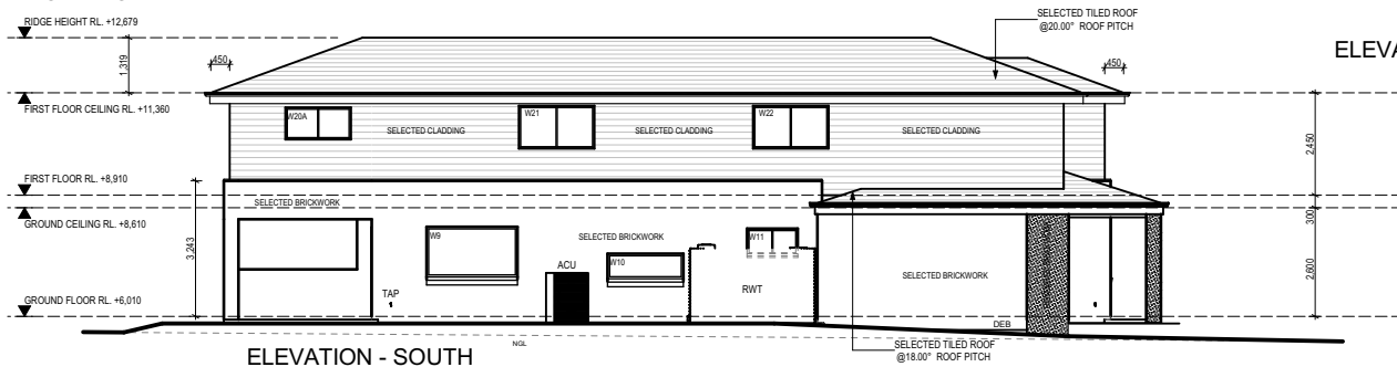
ELEVATION - SOUTH
