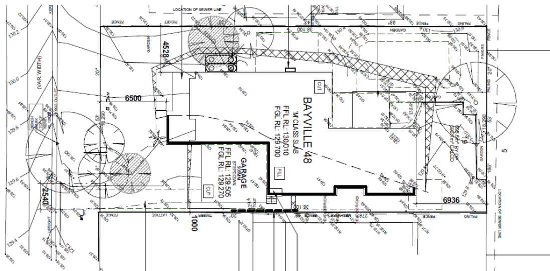
Figure 2: Site plan.
