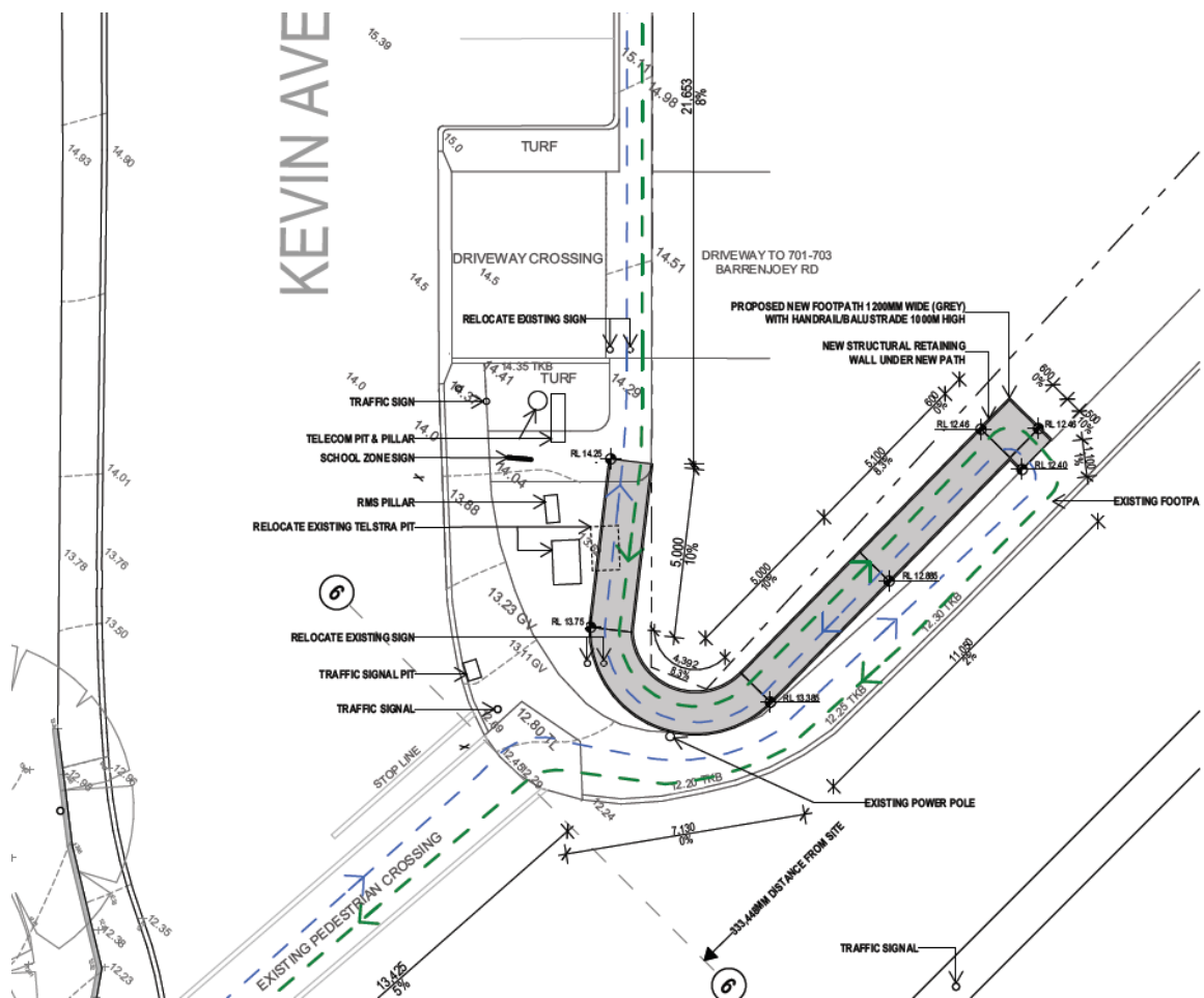
Existing footpath approach to Barrenjoey Road
