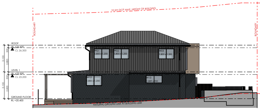
01 WEST ELEVATION 1:250
