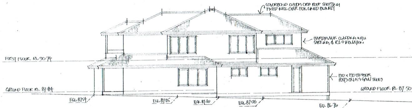
NORTH ELEVATION
