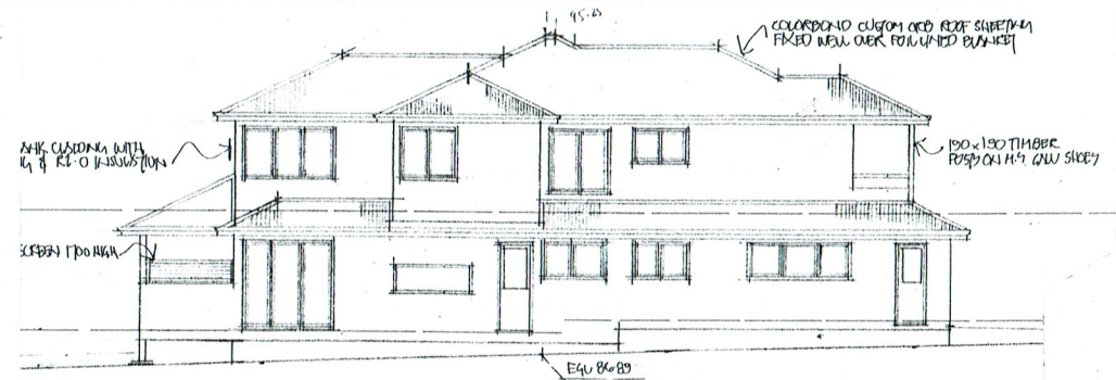
SOUTH ELEVATION
