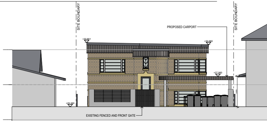
North Elevation
