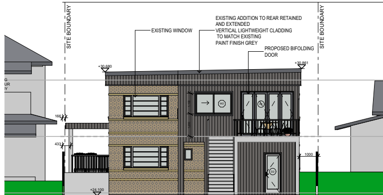
South Elevation
