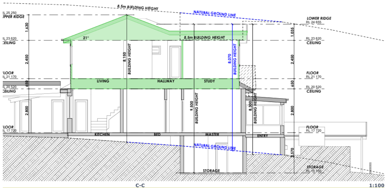
Image 2: Section Drawing
