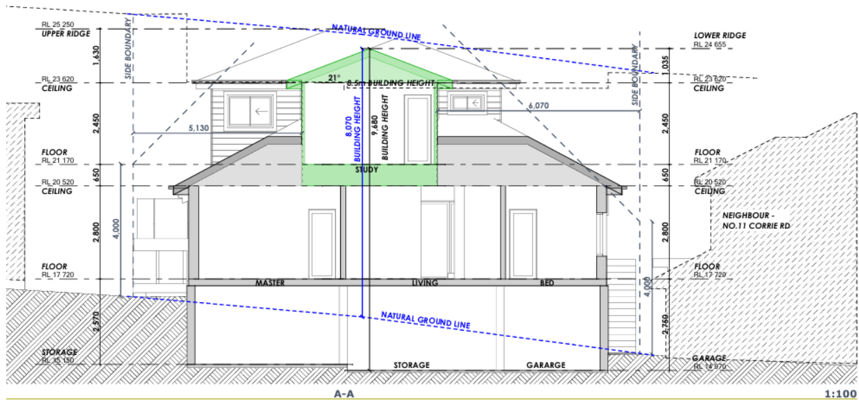
Image 1: Section
