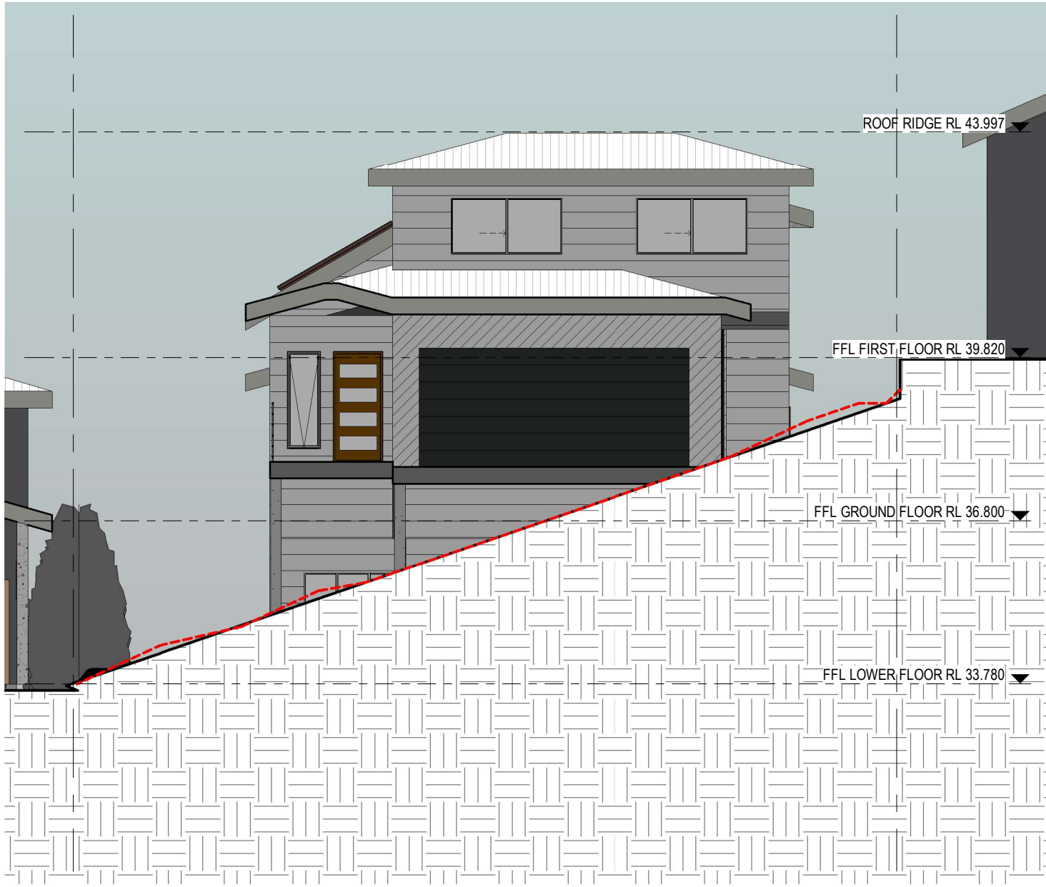
1 SOUTH ELEVATION 1 : 100
