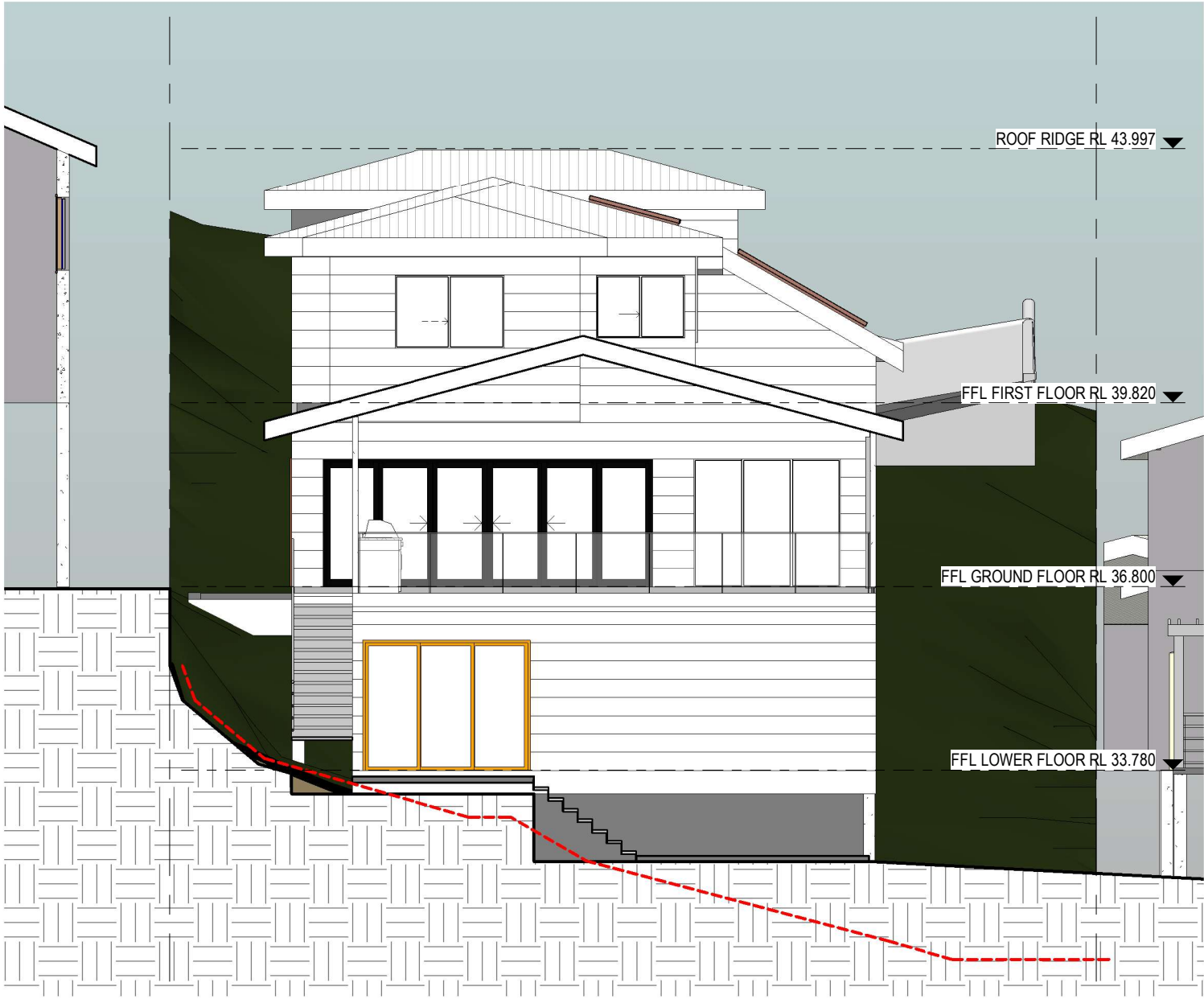
2 NORTH ELEVATION 1 : 100
