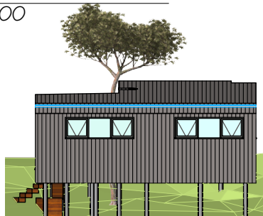
4 EAST ELEVATION 1:200
