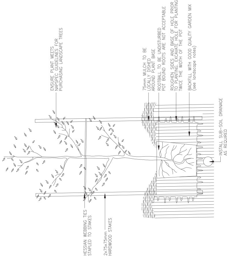
1 TREE PLANTING DETAIL NTS 25litre-75litre pot size
