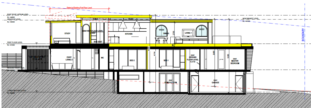
Existing section depicting existing and natural ground level
