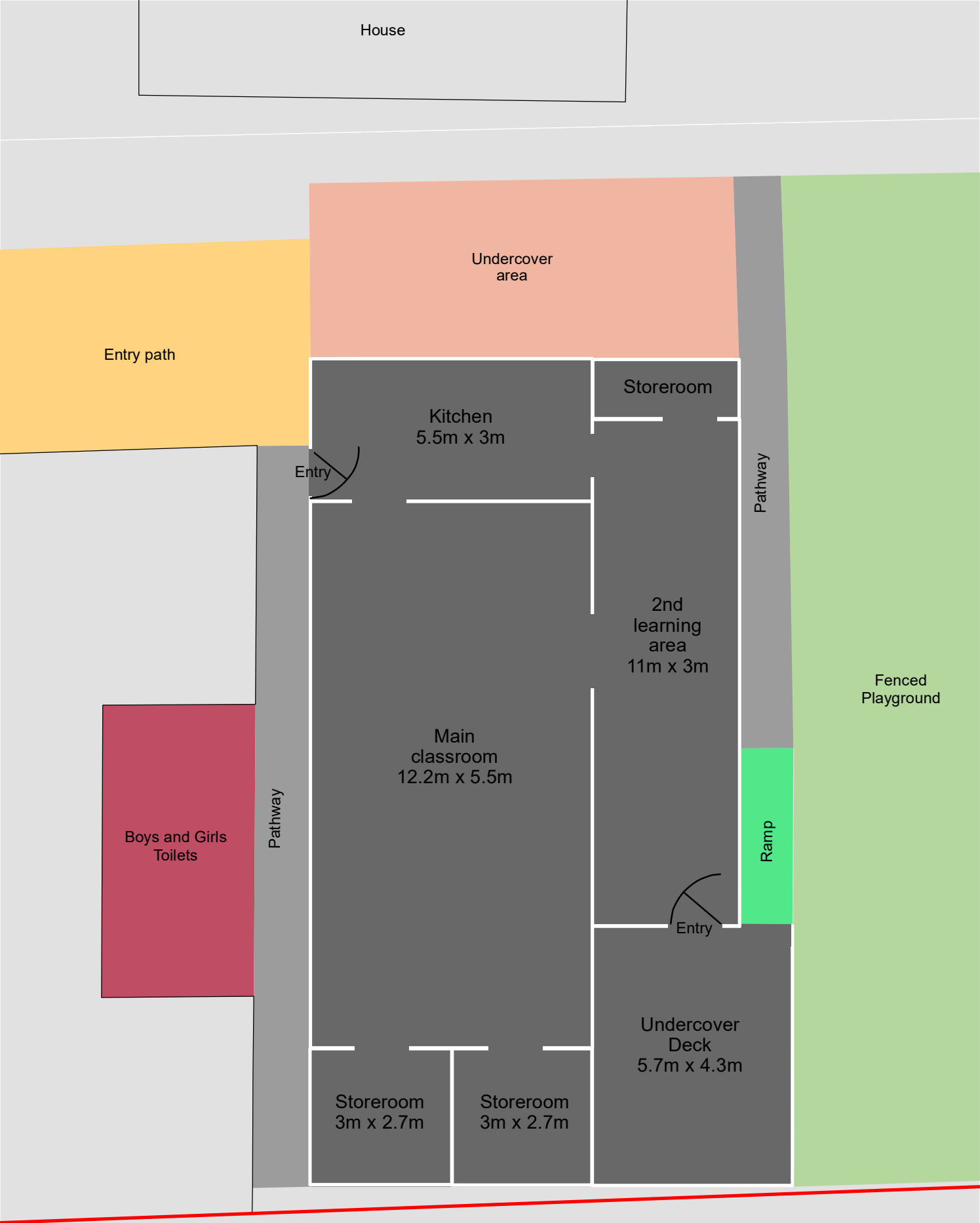
Floor Plan
