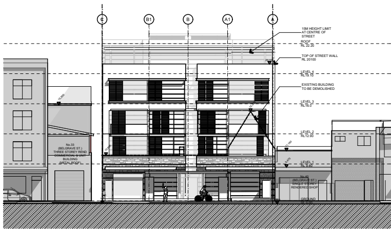
East Elevation
