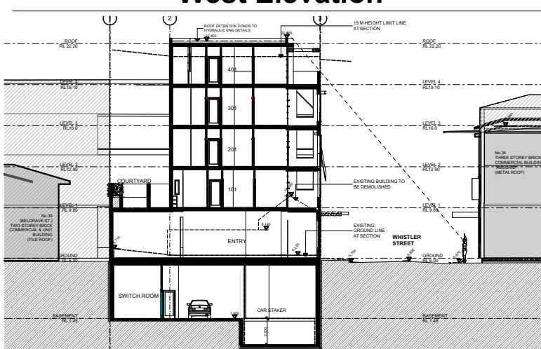
AA Section
