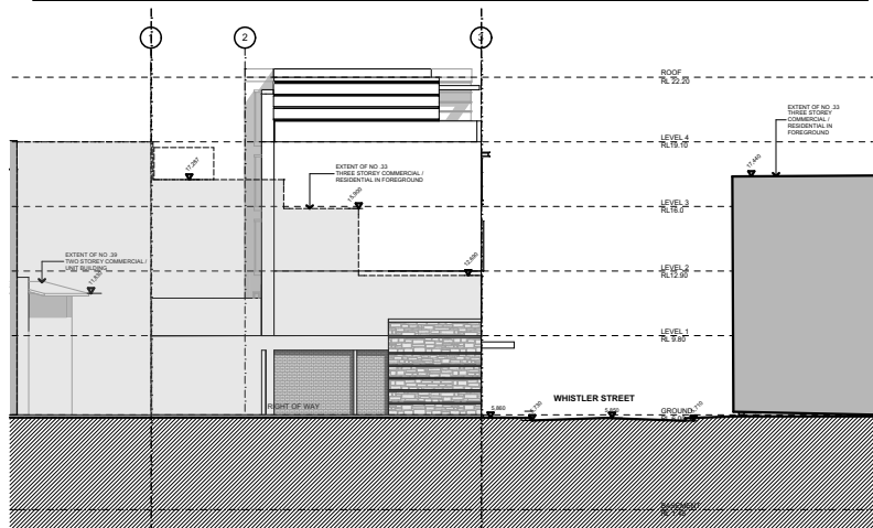
South Elevation
