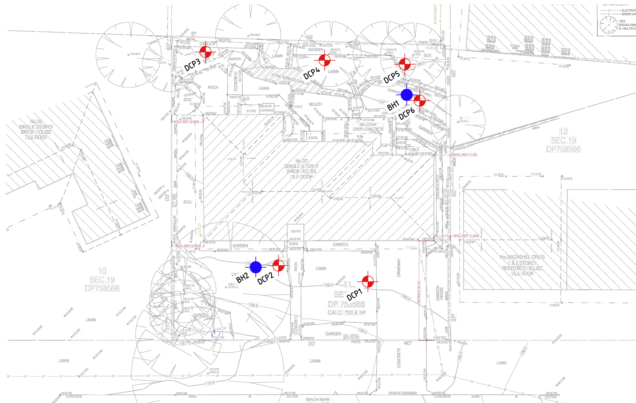
SITE PLAN/GROUND TEST LOCATIONS SCALE NTS
