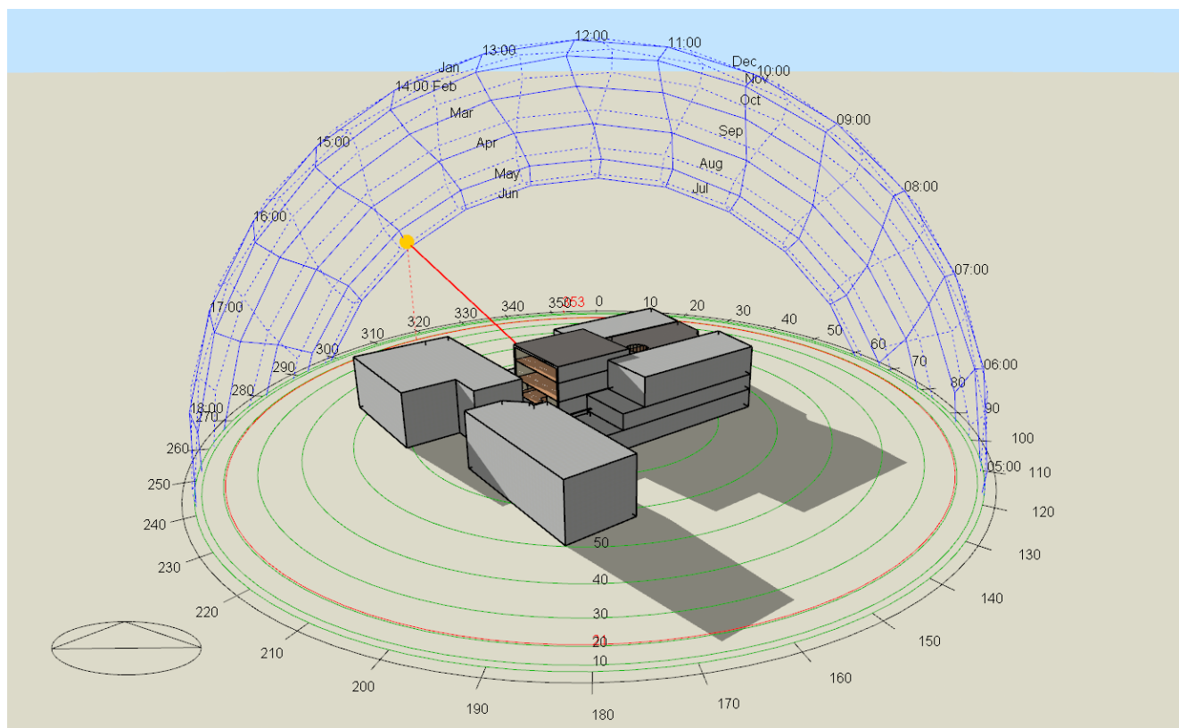
Figure 4. Design Builder Model Geometry.
