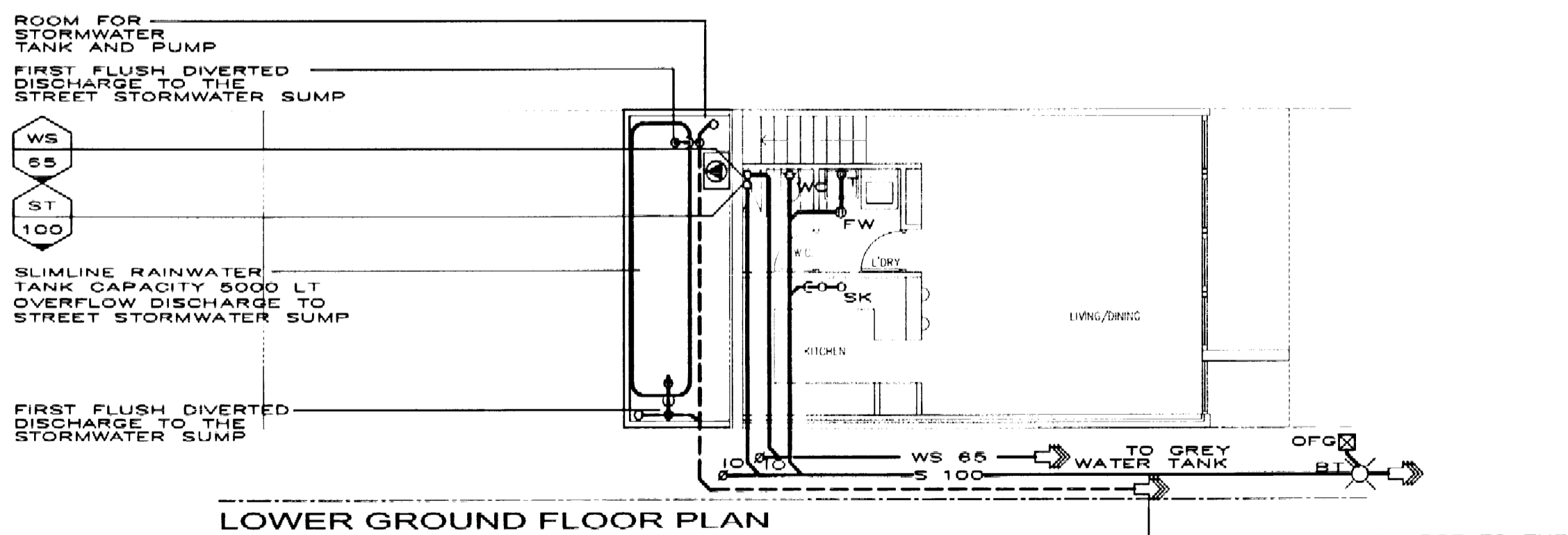
SANITARY PLUMBING DRAINAGE
