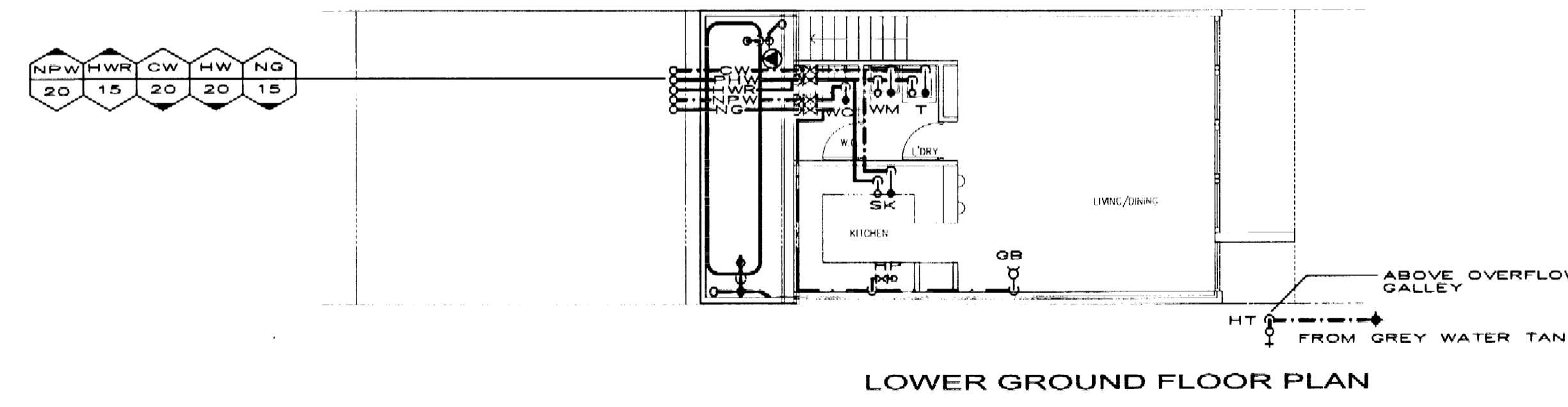
WATER & GAS SERVICES
