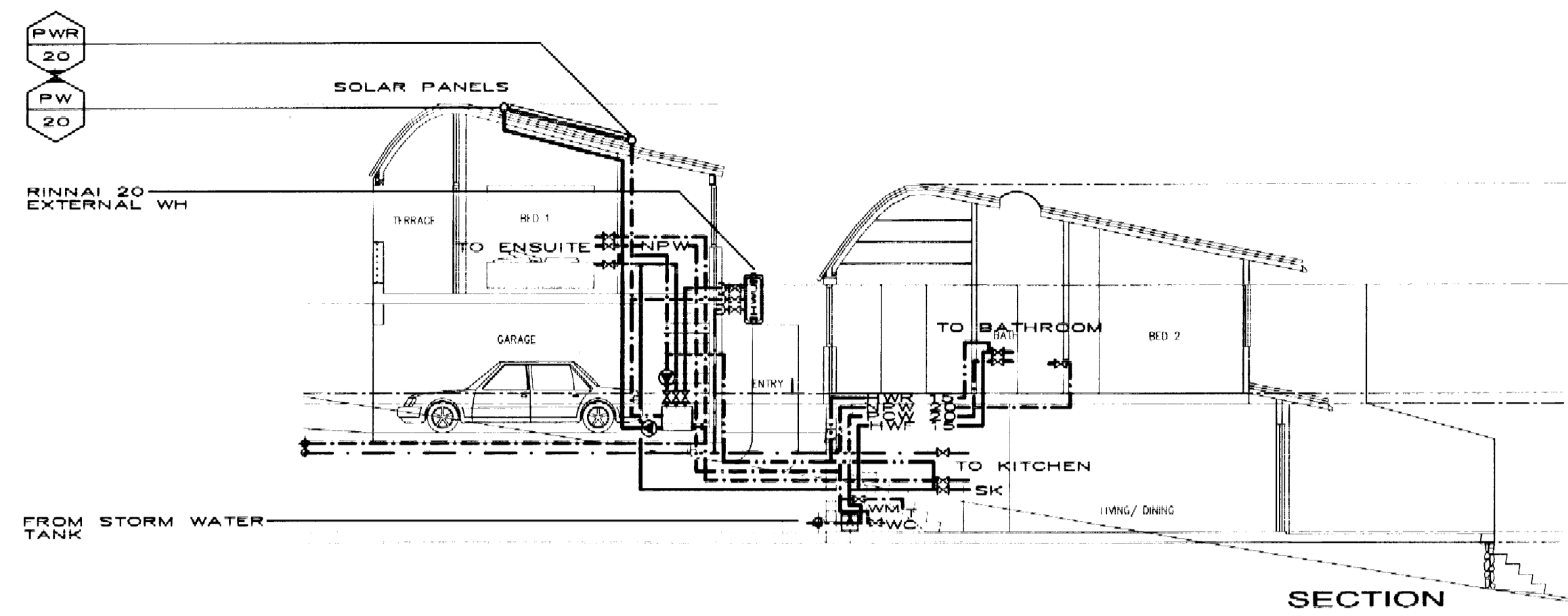
SECTION
