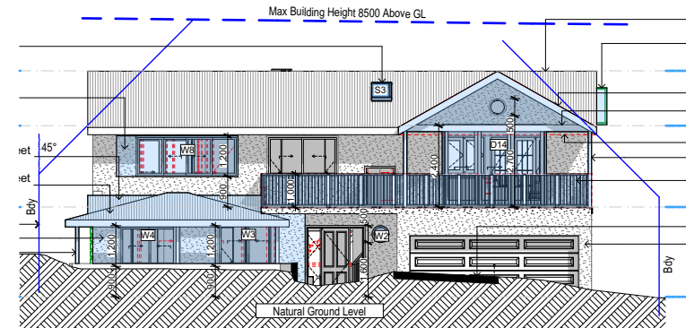
South 1:200
