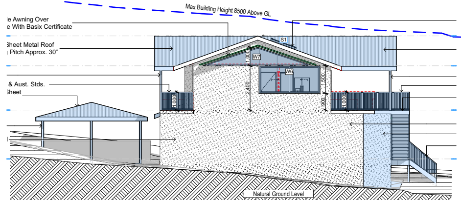
East 1:200
