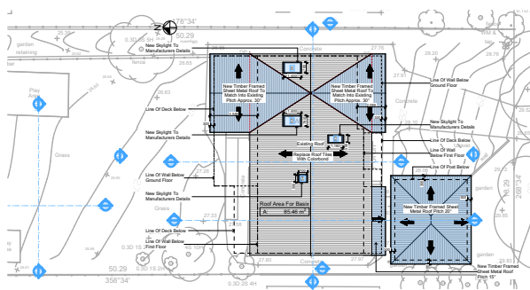
Roof Plan 1:500
