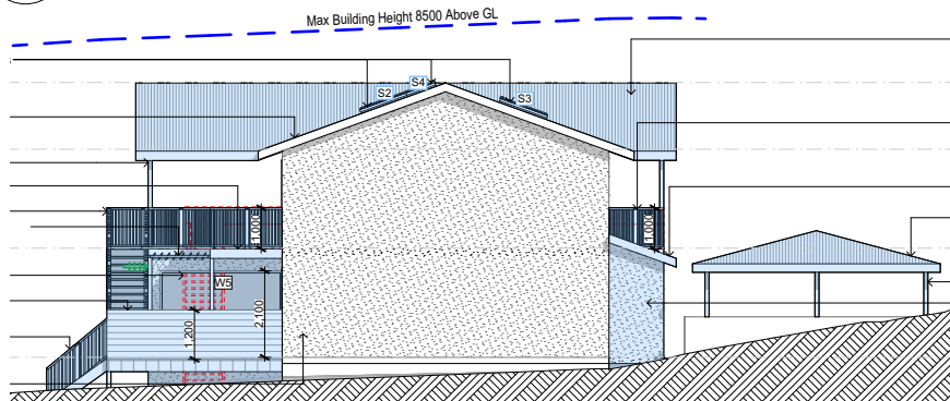
West 1:200
