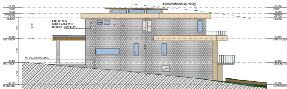
WESTERN ELEVATION
