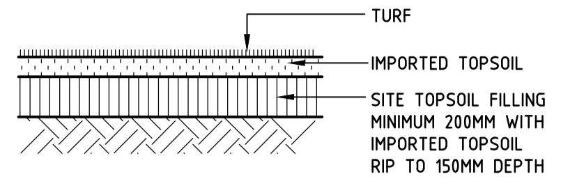
LAWN DETAIL SCALE 1:10
