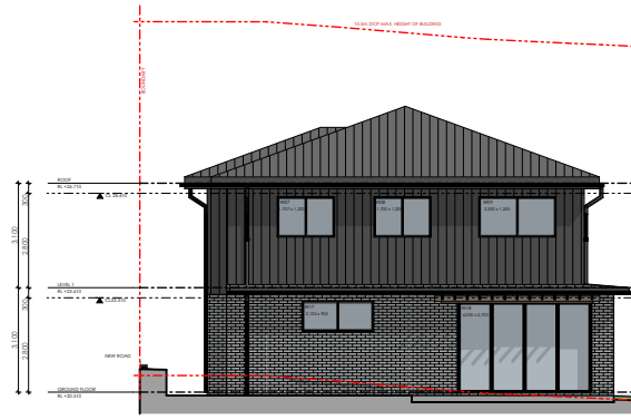
2 EAST ELEVATION 1:250
