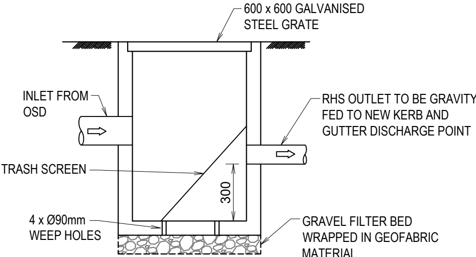
SILT ARRESTOR PIT DETAILS
