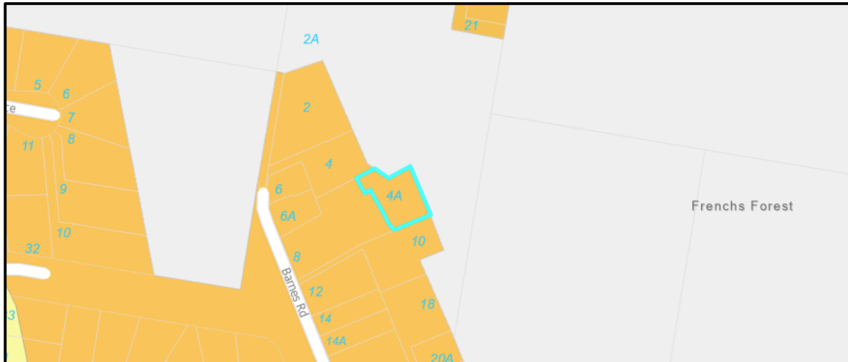
Figure 1. Warringah Landslip Risk Map: 4A Barnes Road, Frenchs Forest NSW (© NBC Maps)
